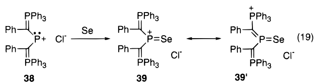
FIGURE 10. Phosphorus cations.
